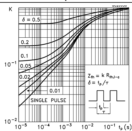
Figure 2. Thermal impedance for TO-220
